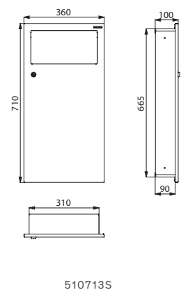
Waste bin with flap 510713S
