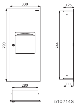
Combi dispenser/bin 10 litres 510714S
