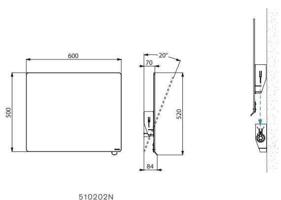
Tilting mirror with white HR Nylon tab handle 510202N For more mirrors and studded pegs see pages 43 - 45.
