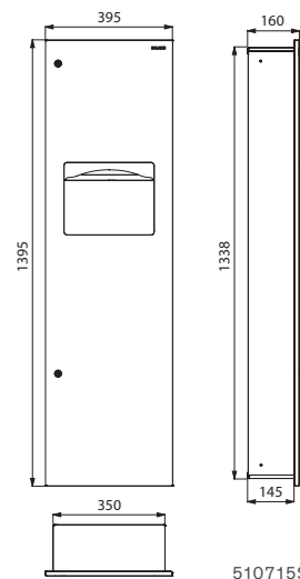
Combi dispenser/bin 30 litres 510715S
