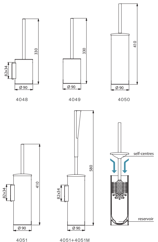
White powder-coated 304 stainless steel, model without lid
