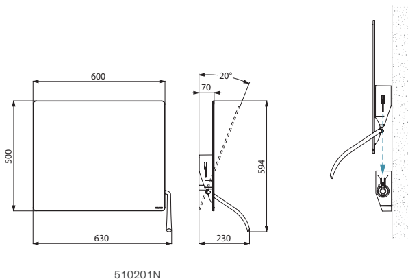
Tilting mirror with long, ergonomic - white HR Nylon lever 510201N For more mirrors and studded pegs see pages 43 - 45.
