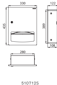
Paper towel dispenser 510712S
