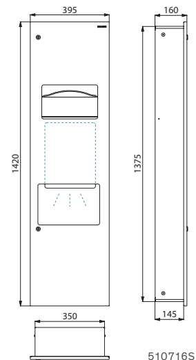
Combi dispenser/bin hand dryer 510716S
