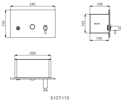
Soap dispenser 510711S
